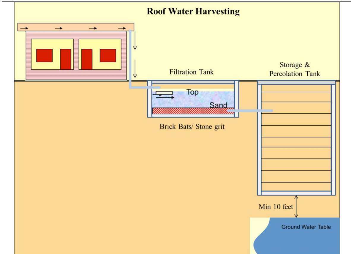
Exhibit 15: Typical Design of Roof Water Harvesting
