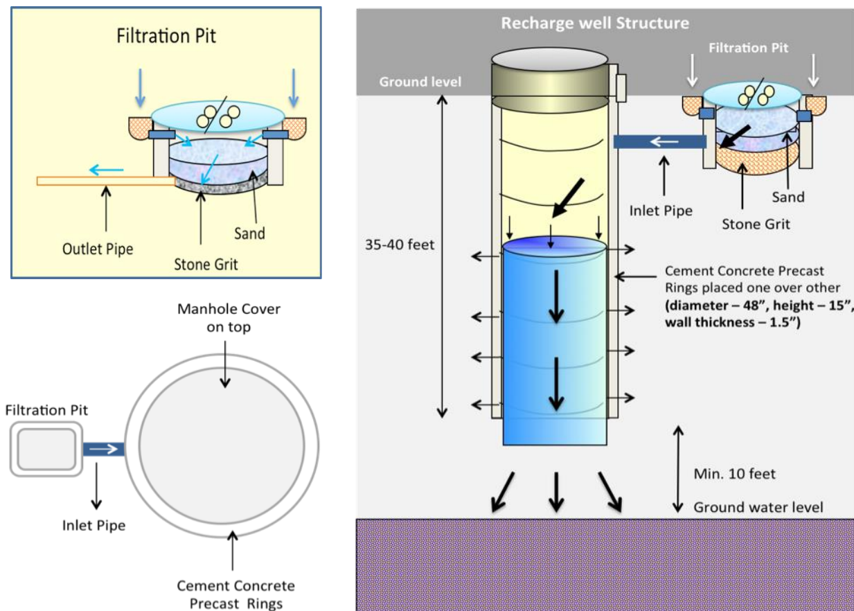
Exhibit 17: Details of proposed recharge well and filtration pit
