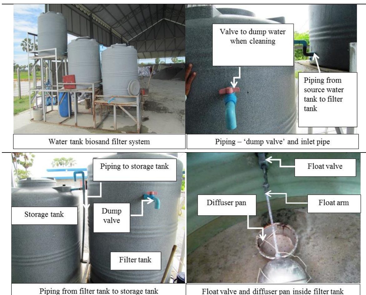
Exhibit 14: Community Water Tank Bio-sand Filter
