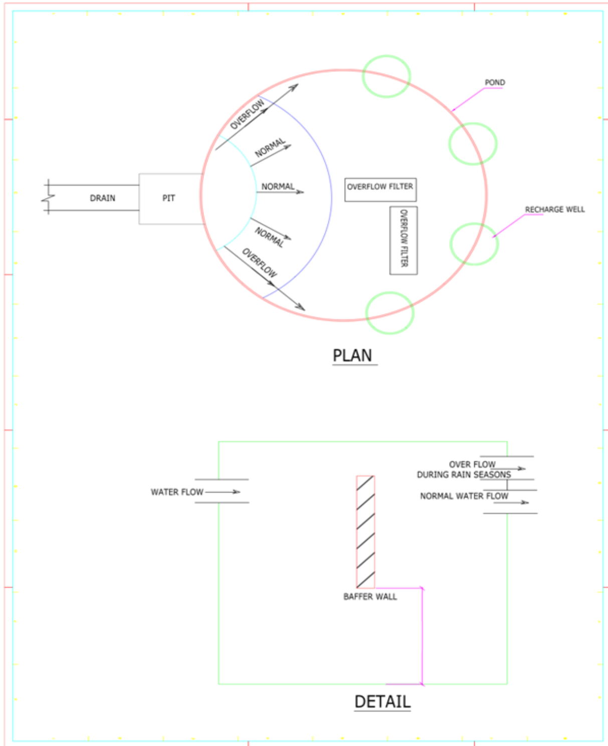
Exhibit 21: Typical Design of Recharge Well for Johad
