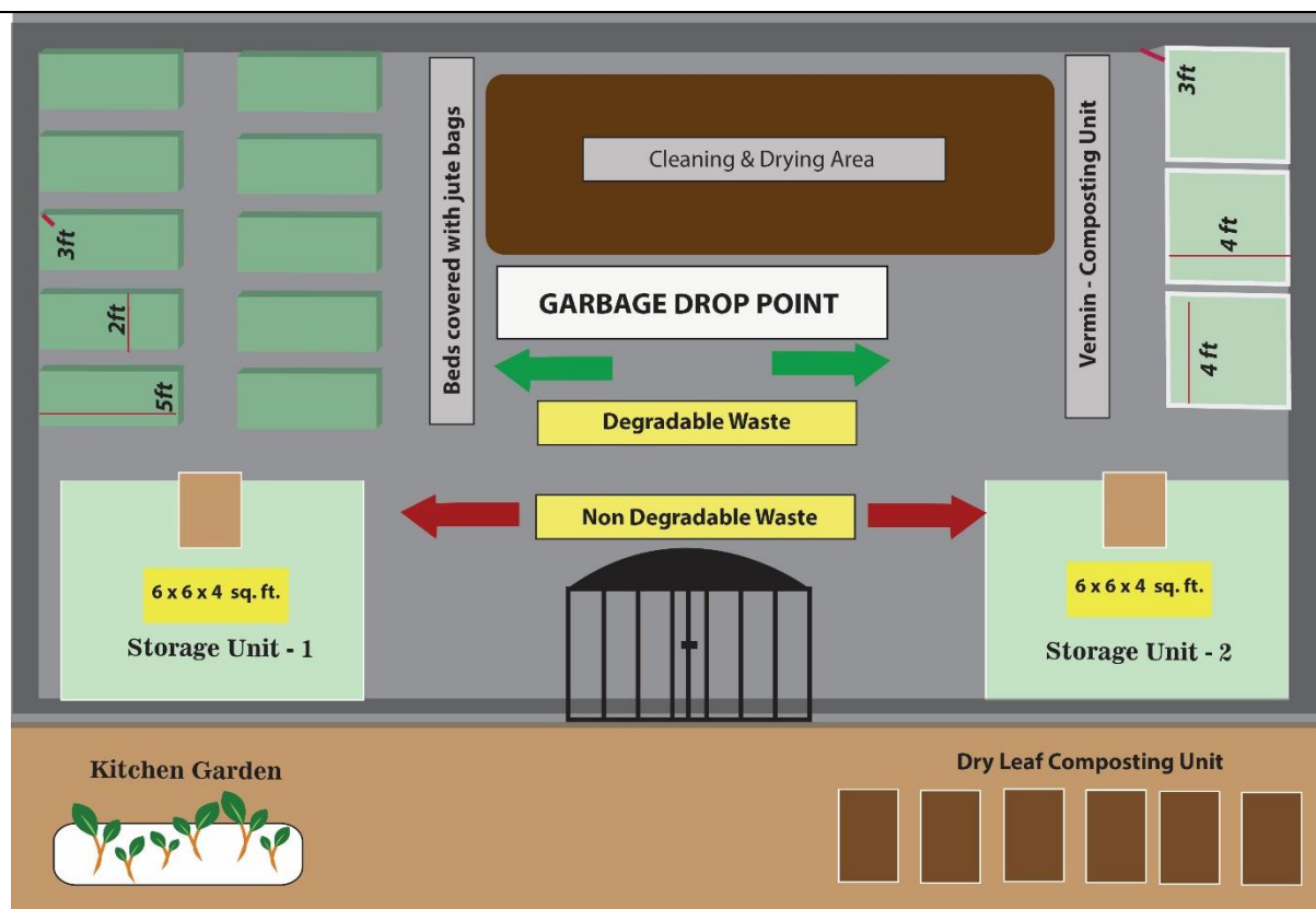
Exhibit 20: Schematic drawing of Resource Recovery Centre at Garhi Harsaru
