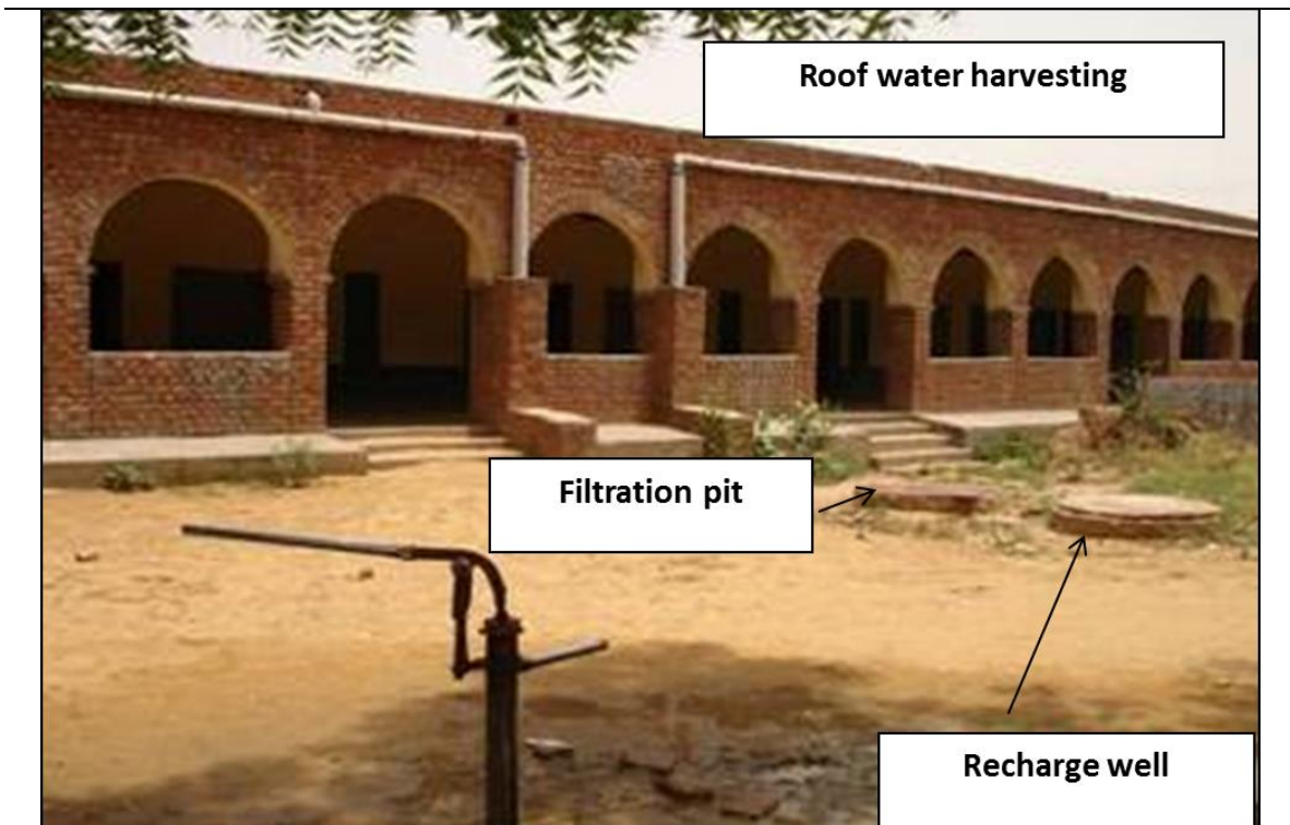
Exhibit 16: Representative image of the proposed rain water harvesting structure
